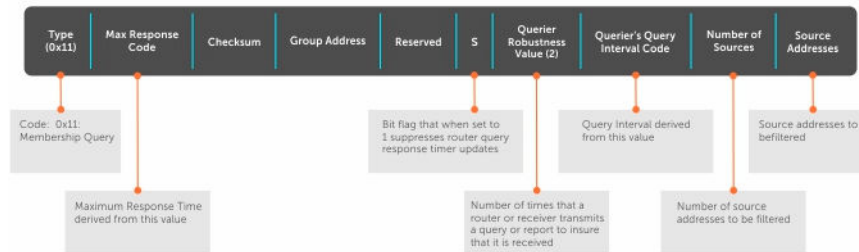
Figure 38. IGMP Version 3 Packet Structure
